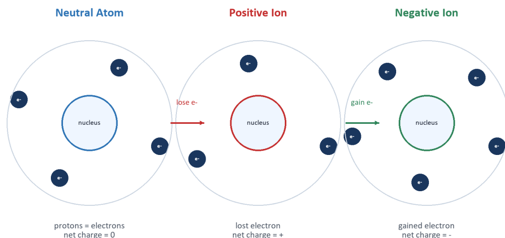
Figure 2. Ion formation through electron loss or gain.
