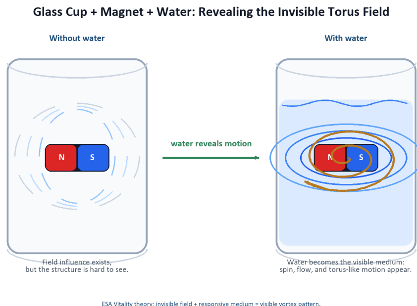
Figure 7. Glass cup, magnet, and water demonstration for invisible torus-field/vortex theory.
