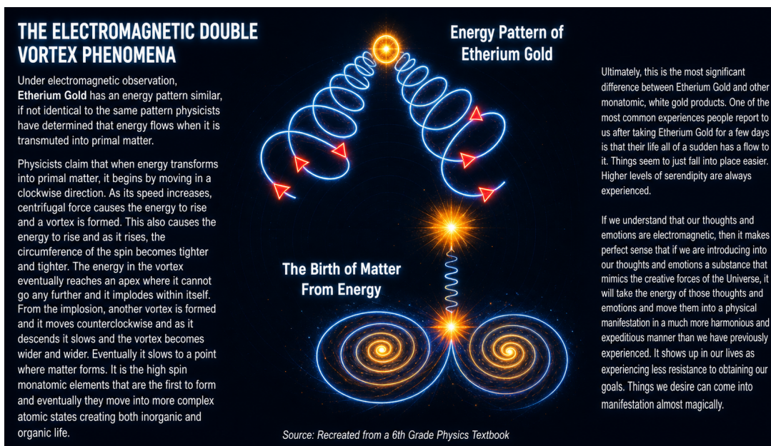
Figure 5. Electromagnetic double healing vortex: an example of the birth of matter from energy using the immaculate concept.
