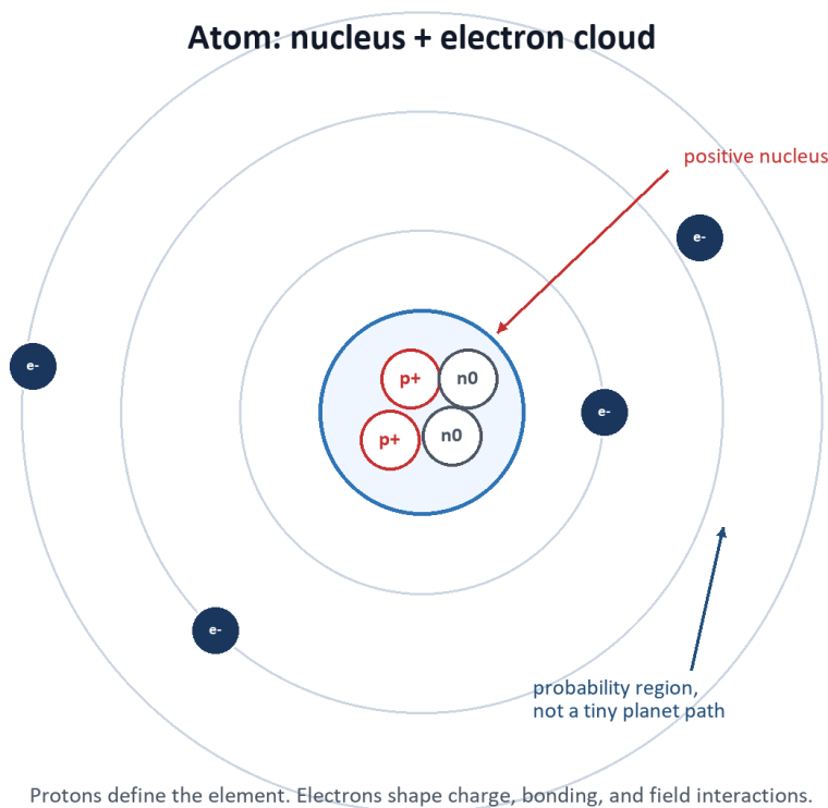
Figure 1. Atom structure: nucleus, protons, neutrons, and electron cloud.
